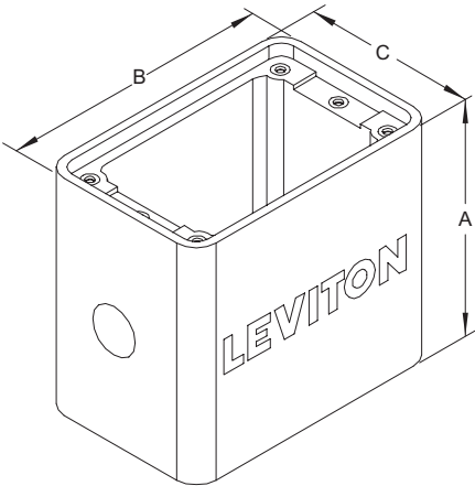
SINGLE-GANG BOX
