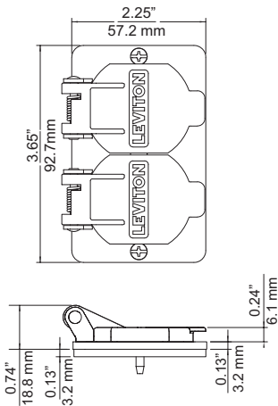
SINGLE-GANG DUPLEX COVERPLATE WITH FLIP-LID TYPICAL
