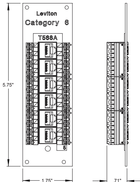
Expansion Board 47611-0C6
