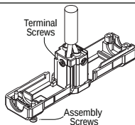
Fig. 3a Straight Blade Connector
