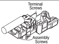
Fig. 3c Angle Plug
