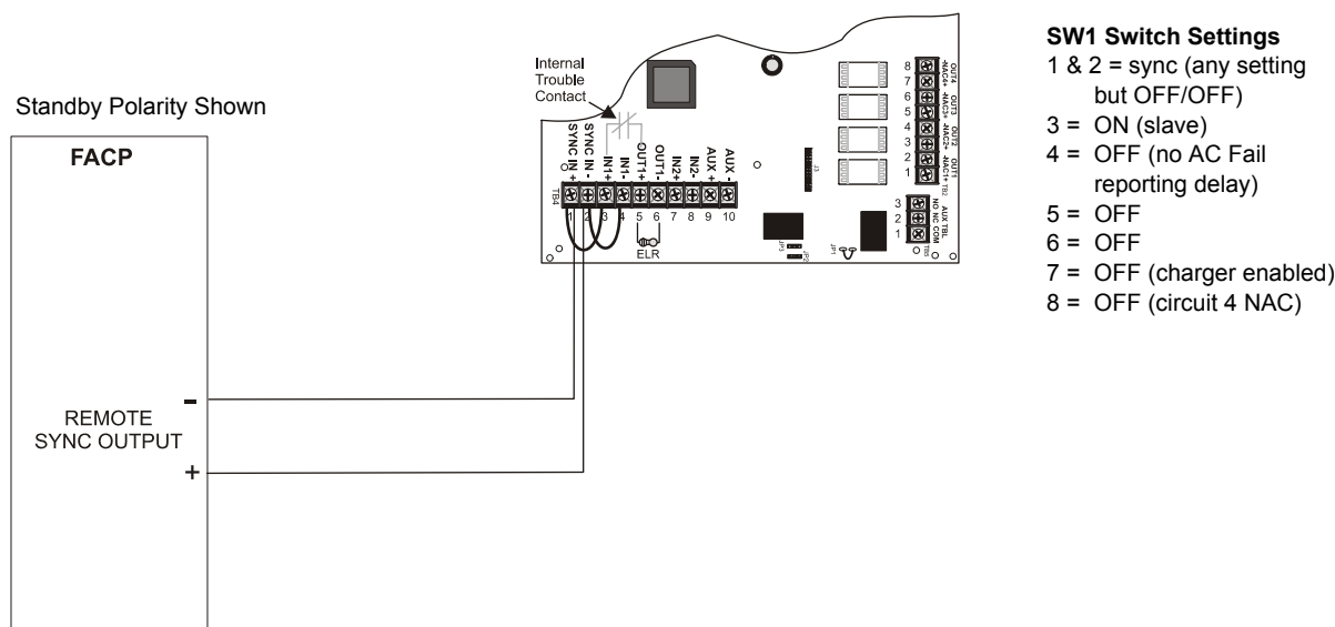
5.5b: Supervised Master/Slave Connections (Remote Sync Source)
