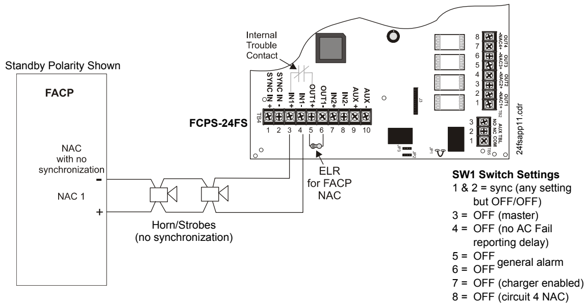
Figure 5.6 Supervised FACP to Master Connections
