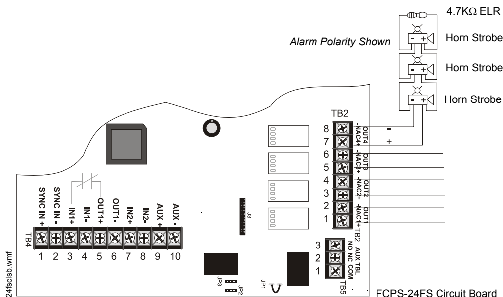
Figure 2.3 NAC Style Y (Class B)
