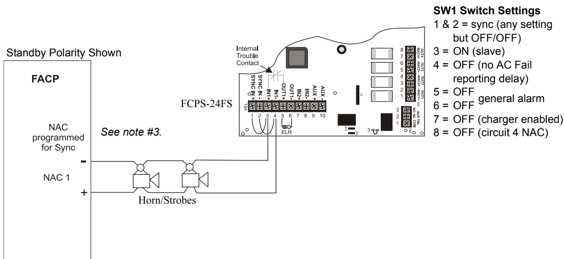
5.5a: Supervised Master/Slave Connections (Filtered, Synchronized NAC Source)
