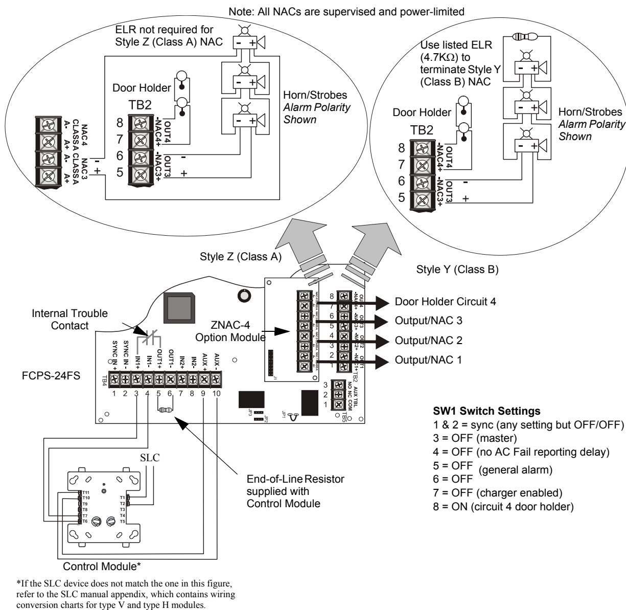
Figure 5.2 Controlling Three NACs and One Door Holder With One Input
