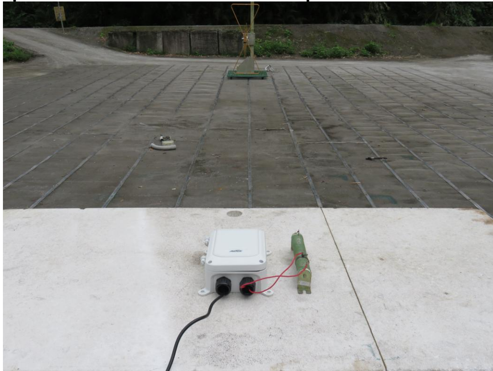
Photograph –Harmonics & Flicker Test Setup
