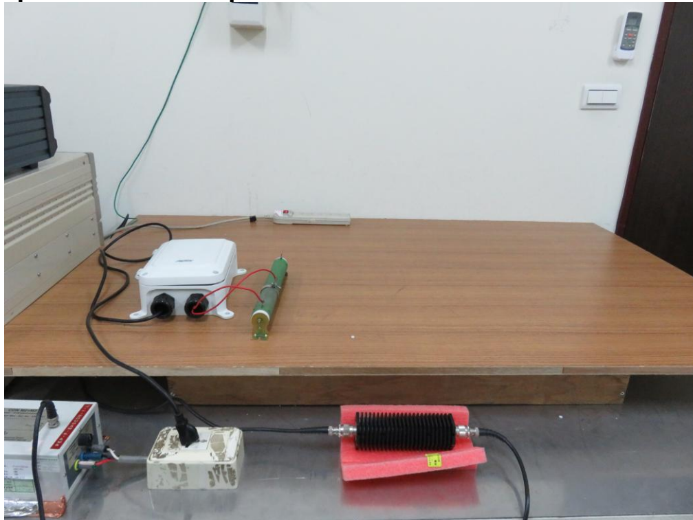
Photograph –PFMF Test Setup
