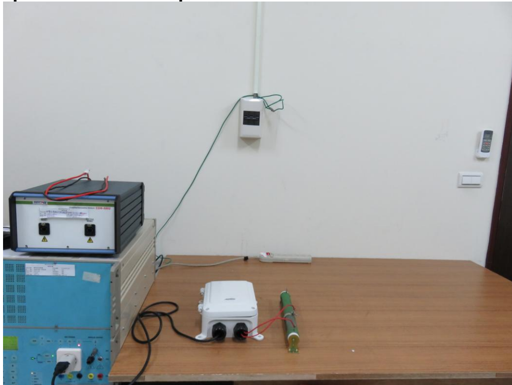
Photograph –EFT Test Setup
