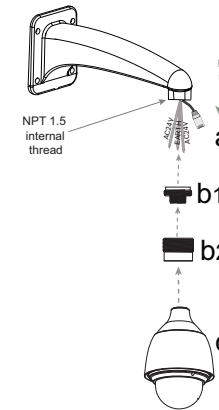
Fig. 2: Example installation: AUTODOME IP 5000 HD camera + G 3/4 to M33 adapter + NPT 1.5 to G 3/4 adapter + third-party wall mount
