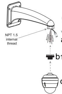
Fig. 1: Example installation: AUTODOME IP 4000 HD camera + NPT 1.5 to G 3/4 adapter + third-party wall mount
