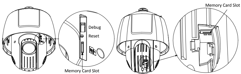
Figure 1-4 Memory Card Slot
