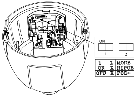
Figure 2-5 PoE+ and Hi-PoE Switch
