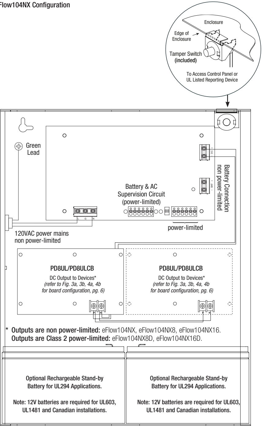
Fig. 7 - eFlow104NX Configuration
