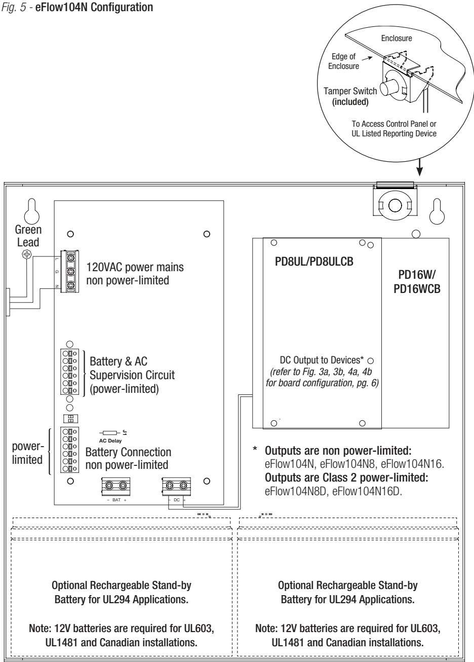
Fig. 5 - eFlow104N Configuration
