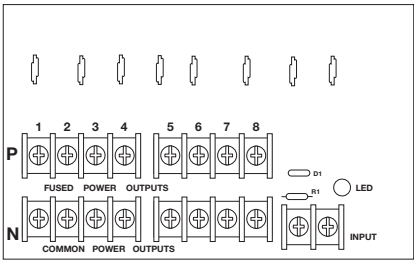
Fig. 3b - PD8ULCB - Power Distribution Board Class 2 Power-Limited Outputs
