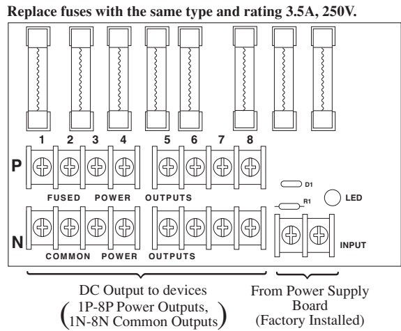
Fig. 3a - PD8UL Power Distribution Board
