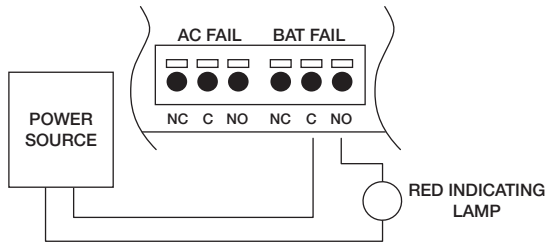
Fig. 2 - Battery trouble indication - For Canadian use, a red indicating lamp must be visible from the exterior of this enclosure. Wire one leg of a UL Listed, power-limited power source to the indicating lamp. Wire the second leg of the power source to the indicating lamp in series with the battery fail relay contact terminals marked [BAT FAIL - C, NO] (Fig. 2, pg. 6).
