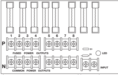
Fig. 3a - PD8UL Power Distribution Board
