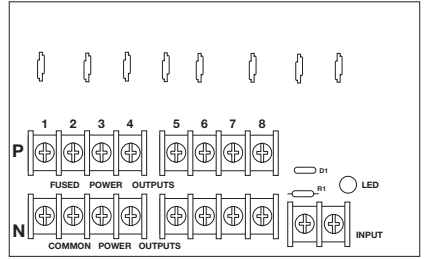
Fig. 3b - PD8ULCB - Power Distribution Board
