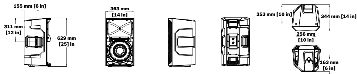
Figure 7.2: ELX200-12 dimensions
