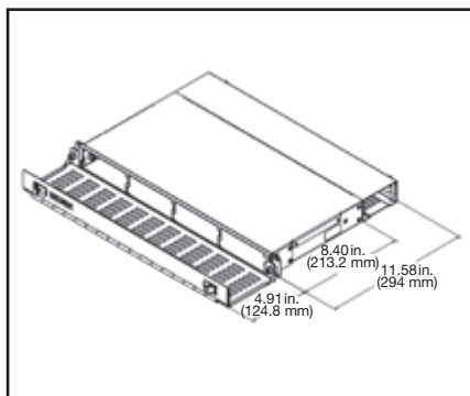
FX UHD 1U Housing
