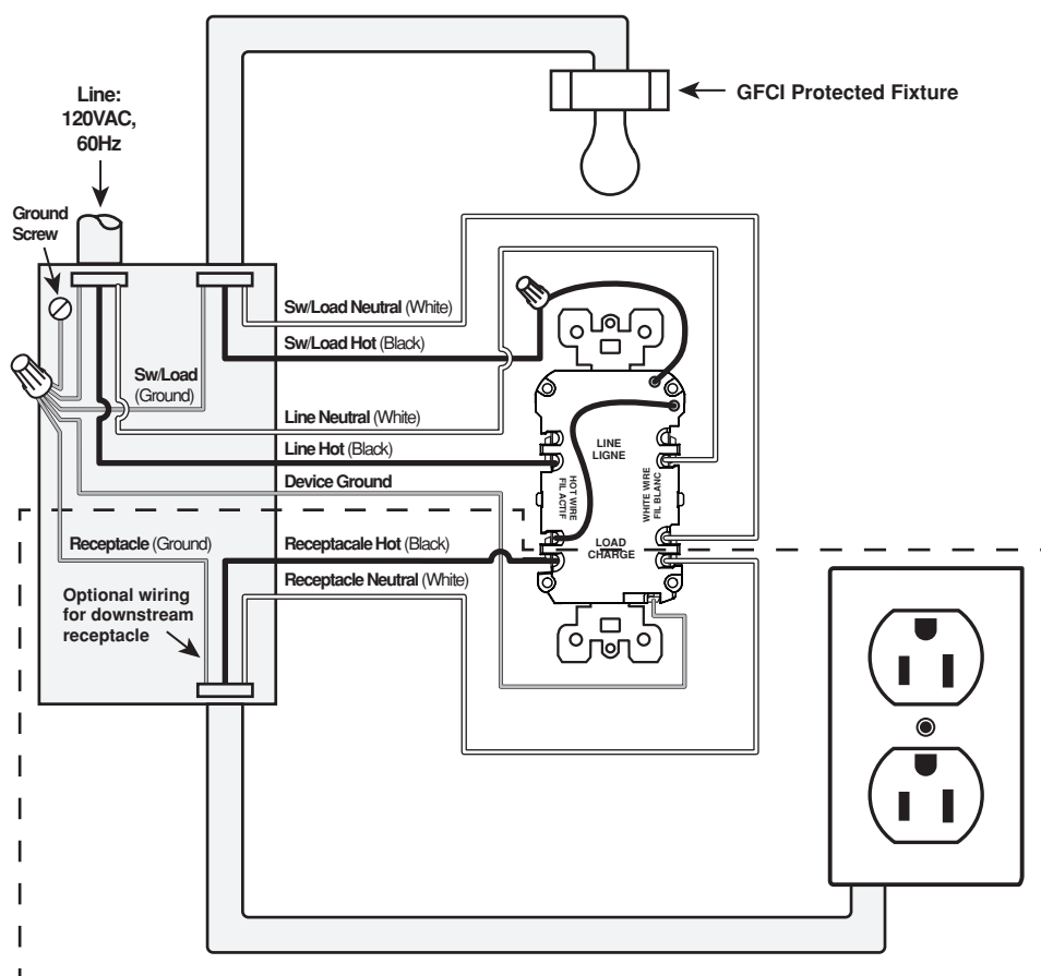
Combination GFCI/Switch with switched load GFCI protected
