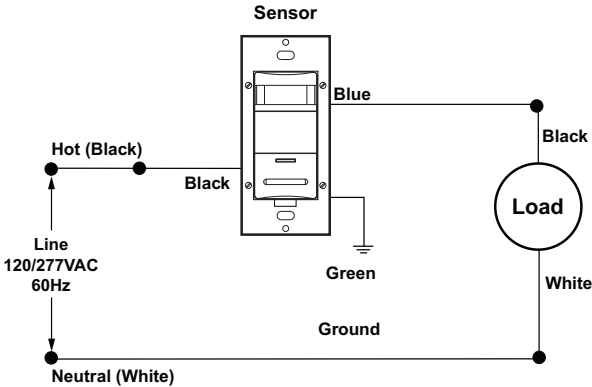
Wiring Diagram 1 - Single Control Application
