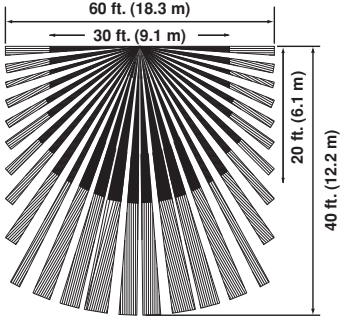
Figure 1 - Field-of-View (Horizontal)
