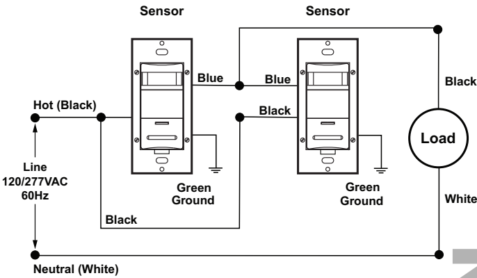
Wiring Diagram 2 - Two Location Control Application
