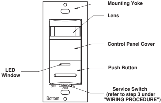
Figure 2 - Sensor Features
