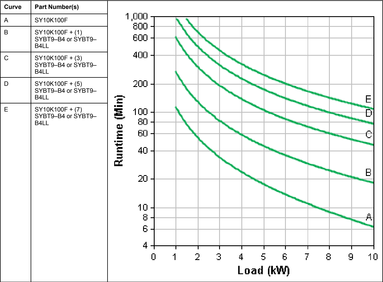
Symmetra PX 10 kW Scalable to 100 kW Battery Run-Times (Minutes)
