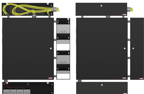
Typical battery/wiring setup with Trove3 Enclosure (not included).
