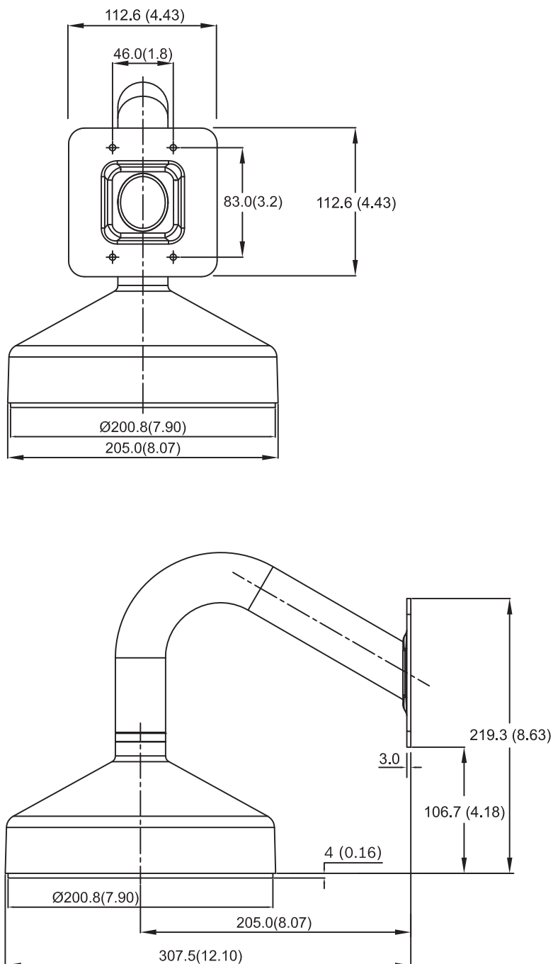
Figure 4.1 VDA-832FHD-WMT dimensions
