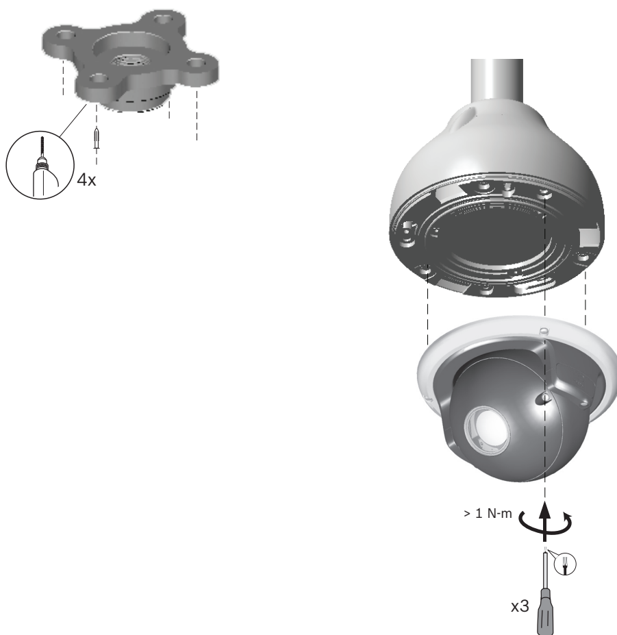
Figure 3.2 Pendant Pipe Mount installation
