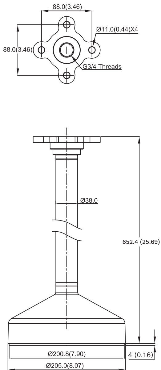
Figure 4.2 VDA-832FHD-PMT dimensions
