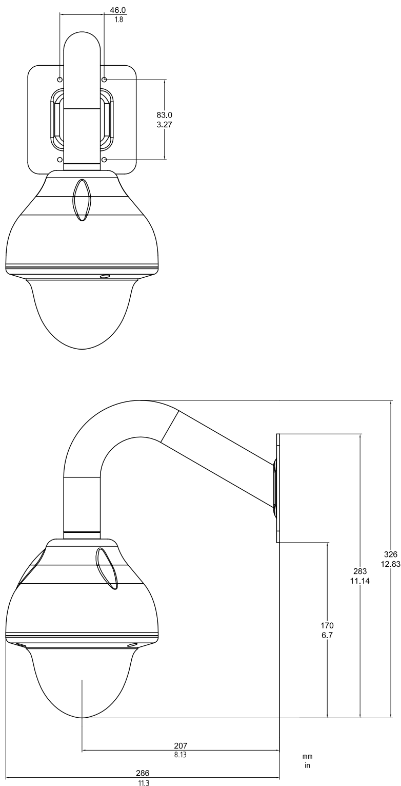
Figure 4.1 VDA-WMT-DOME dimensions
