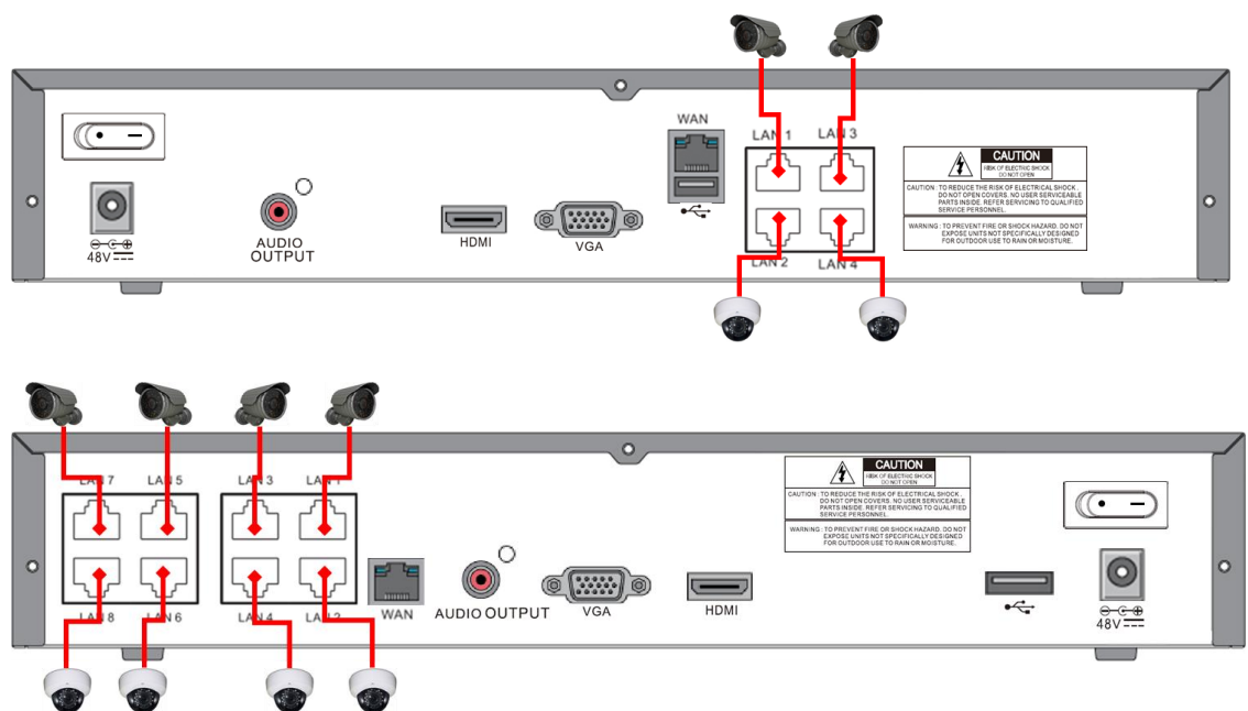
Figure 2.5.1.1 IP Camera Connection Diagram (N4NSL, N8NSL)
