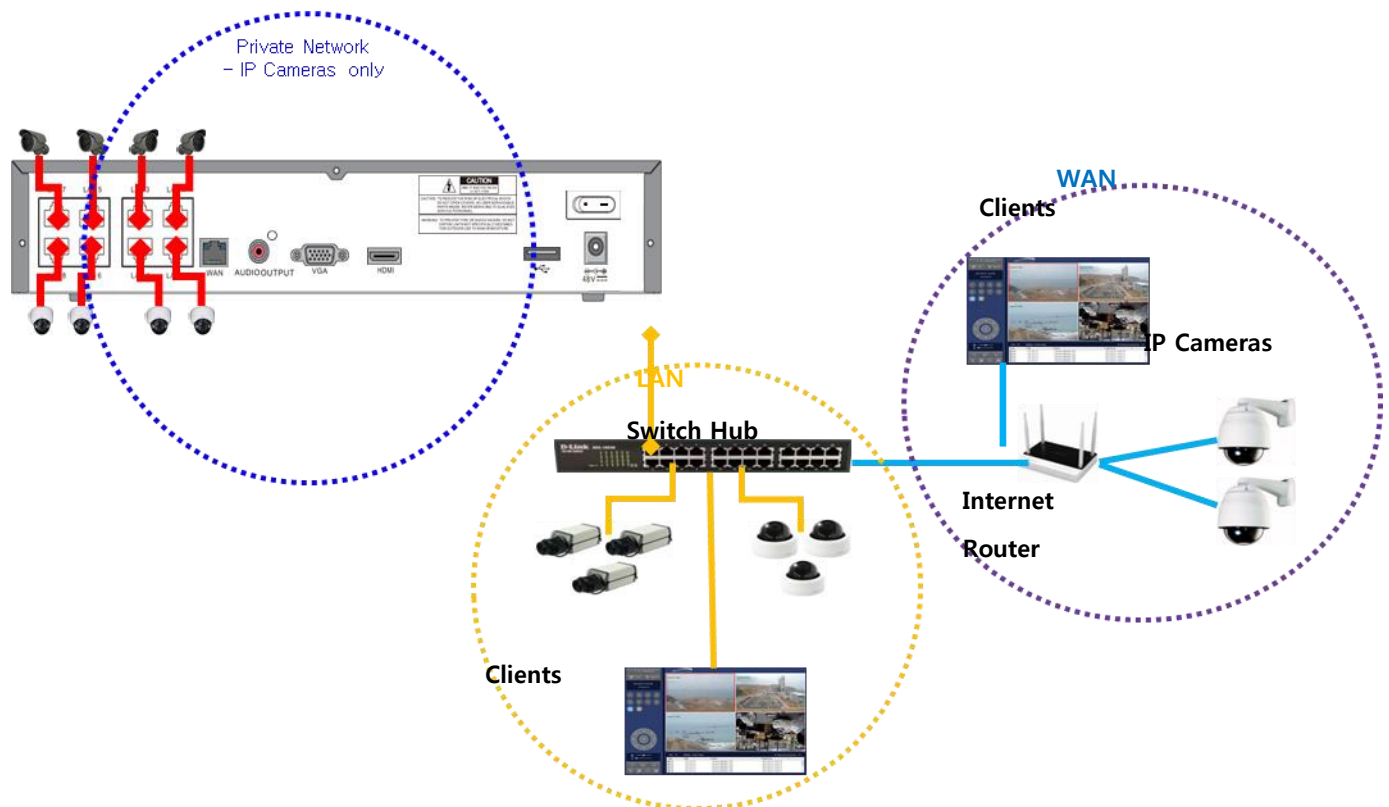
Figure 2.5.1.2 IP Camera Connection Diagram (NSL Series)
