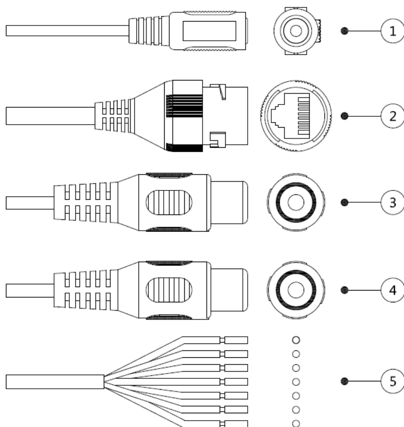
Figure 1-1 Cable list
